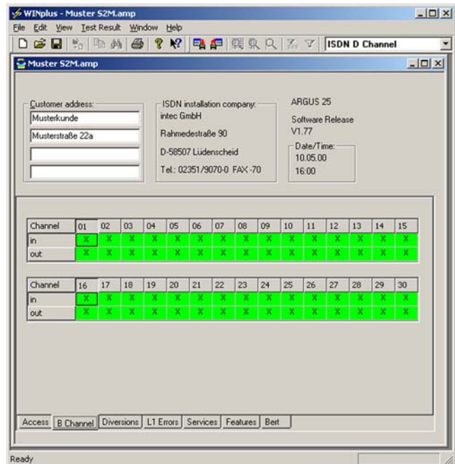
(Display of the PRI B-channel configuration with WINplus)
